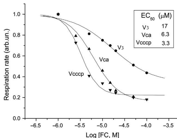
FIGURE 16.2 Effects of FC on respiration of rat liver MCh. Dependence of respiration rate activated by ADP ( V_3 ), calcium transport ( V_{Ca} ), and protonophore CCCP ( V_{cccp} ) upon concentration of FC. Substrates: pyruvate + malate.
