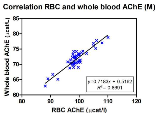
FIGURE 65.3 Correlation between RBC and whole blood AChE.
