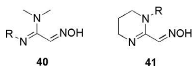
FIGURE 72.30 Amidine oximes from a study in the United States (Kalisiak et al., 2011).
