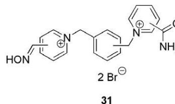
FIGURE 72.25 Mono-oxime-mono-carbamoyl bispyridinium xylene-linked reactivators (Musilek et al., 2010).
