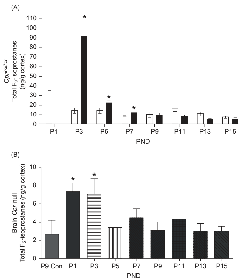
FIGURE 20.3 In utero exposure to B(a)P aerosol (100 \mu\text{g}/\text{m}^3 ) produces an approximate 10 \times higher concentration of F 2 -isoprostanes on P3 in B(a)P-exposed Cpr lox/lox offspring as compared to B(a)P-exposed brain-Cpr-null offspring. (A) F 2 -isoprostanes levels derived from control (white bars) and B(a)P-exposed Cpr lox/lox (black bars) offspring neocortex. (B) F 2 -isoprostanane levels for derived from control PND9 (white bar) and B(a)P-exposed (black bars) brain-Cpr-null offspring neocortex. Due to the limited number of control offspring, only PND9 was used for time points in favor of reserving pups for behavioral determinations in later-life. * P < 0.05 versus Control.
