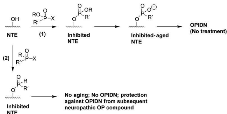
FIGURE 63.2 Reaction of NTE with an organophosphonate in pathway (1) yields a phosphonylated (inhibited) enzyme, which can undergo net loss of an R-group to yield an inhibited and aged enzyme. Inhibition alone does not produce OPIDN; both inhibition and aging are required, and there is no treatment for the neuropathy. Reaction of NTE with an organophosphinate in pathway (2) yields a phosphinylated (inhibited) enzyme, but because of the stability of the C–P bonds linking the R- and R'-groups to phosphorus the phosphinyl moiety on NTE does not undergo aging, so that OPIDN does not occur. Inhibition of NTE with a nonaging inhibitor is not biologically inert—it protects against subsequent exposures to neuropathic (ageable) NTE inhibitors. R, R' = substituted or unsubstituted alkyl or aryl groups, which can be different or equivalent. X = primary leaving group (e.g., fluoride). Source: Reproduced with permission from Richardson and Makhaeva (2014).
