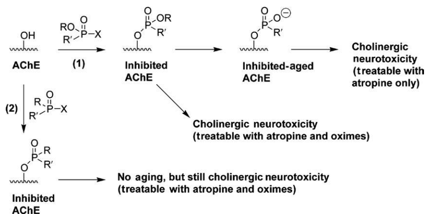
FIGURE 63.1 Reaction of AChE with an organophosphonate in pathway (1) yields a phosphonylated (inhibited) enzyme, which can undergo net loss of an R-group to yield an inhibited and aged enzyme. Inhibition alone produces cholinergic toxicity that is treatable with both atropine to counteract excess acetylcholine at muscarinic acetylcholine receptors and oximes to reactivate AChE. Aging does not change the type of toxicity, but it renders the enzyme intractable to reactivation, so that treatment with oximes becomes ineffective. Reaction of AChE with an organophosphinate in pathway (2) yields a phosphinylated (inhibited) enzyme and produces cholinergic toxicity, but because of the stability of the C–P bonds linking the R- and R'-groups to phosphorus, the phosphinyl moiety on AChE does not undergo aging, so that both atropine and oximes can be used in therapy. R, R' = substituted or unsubstituted alkyl or aryl groups, which can be different or equivalent. X = primary leaving group (e.g., fluoride). Source: Reproduced with permission from Richardson and Makhaeva (2014).
