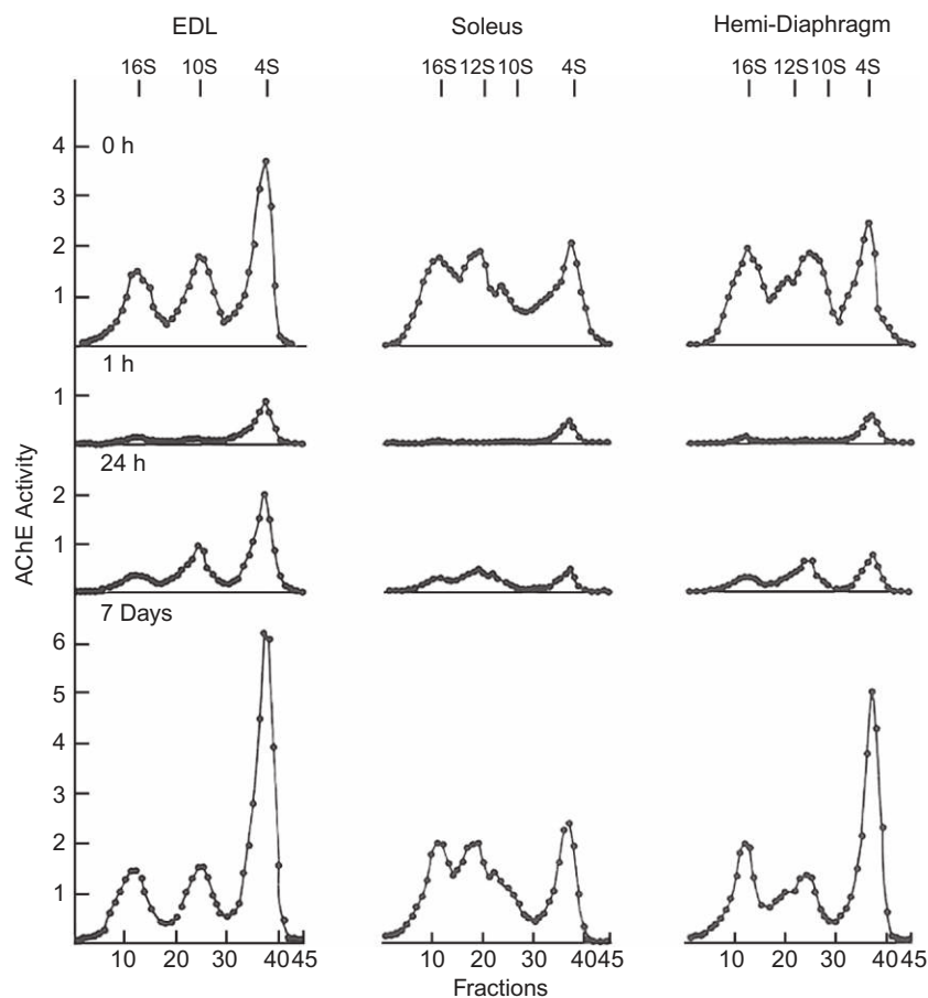
FIGURE 40.3 Representative profiles of the activity of the AChE molecular forms in the EDL, SOL, and hemidiaphragm muscles from rats following an acute, sublethal injection of VX (12 µg/kg, s.c.). For further details, see Figure 40.1 .
