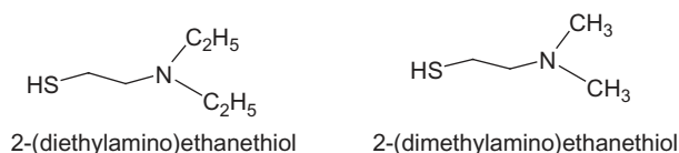
FIGURE 62.10 The chemical structures of 2-(diethylamino)ethanethiol and 2-(dimethylamino)ethanethiol.
