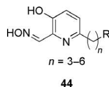
FIGURE 72.33 Reactivators with 3-hydroxy-2-pyridinealdoxime moiety and variable PSL (Renou et al., 2013).
