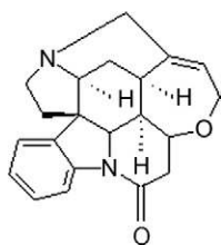
FIGURE 17.1 Structural formula of strychnine.
