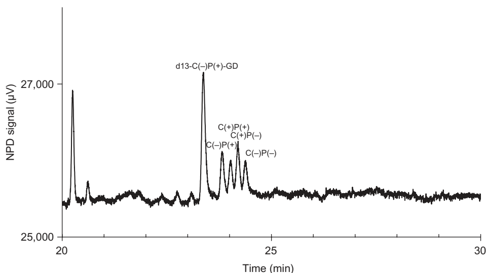
FIGURE 61.3 Typical separation of the stereoisomers of soman and internal standard. d_{13}\text{-C(-)P(+)-soman} using the 2D-GC configuration. Source: Trap and van der Schans (2007) .
