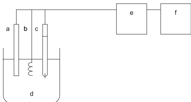
FIGURE 62.2 An experimental setup for the operation of electrochemical biosensors. (a) Biosensor, (b) counter electrode, (c) reference electrode, (d) sample solution, (e) potentiostat, and (f) recorder.
