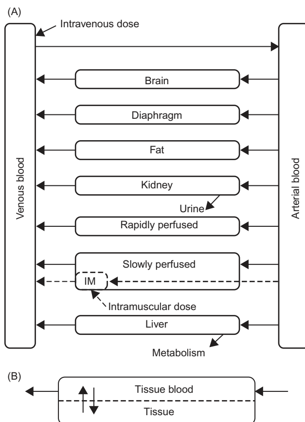
FIGURE 69.1 PBPK model schematic of the distribution of the oxime TMB-4 in rats and humans. Each tissue compartment depicted in schematic A includes diffusion limitation as shown in schematic B (Sterner et al., 2013).
