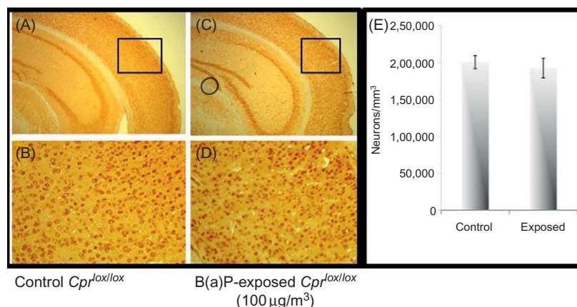
FIGURE 20.8 Post-behavior characterization of neocortical cytoarchitecture. Coronal sections of adult neocortical sections from Cpr lox/lox offspring were analyzed for cytoarchitecture by immunohistochemical staining for NeuN. Neocortical neurons were counted in Cpr lox/lox offspring that had not been exposed to B(a)P in utero (A, low magnification; B, higher magnification) and compared to Cpr lox/lox offspring that were exposed to the B(a)P in utero (C, 4 × -low magnification; D, 20 × -high magnification). (E) It shows the plot resulting from stereological analysis of neocortical neurons subsequent to application of a two-tailed t -test. As can be seen, no significant differences in the density of neocortical neurons is observed as a result of in utero exposure to B(a)P aerosol.
