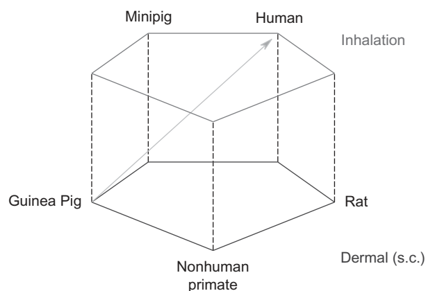
FIGURE 58.2 Schematic illustration of combined interspecies and route-to-route extrapolation. The arrow represents the extrapolation of guinea pig subcutaneous exposure data to human inhalation exposure situations.
